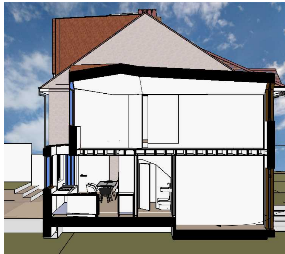
Section view through garage extension
